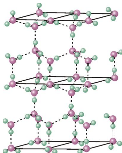
Figure 2.43 Arrangement of H 2 O molecules in ice
