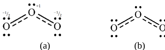
Figure 2.34 (a) Resonance hybrid structure of the O_3 with charges (b) Resonance hybrid structure of the O_3 without charges on terminal/ central atom(s)
