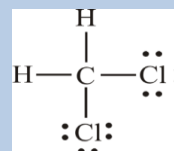
Lewis dot-dash structure
