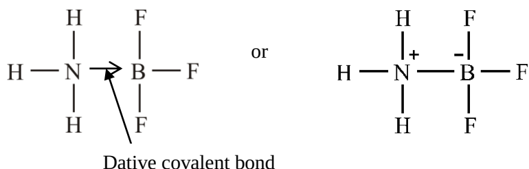
Figure 2.6 Dative covalent bond ( \text{H}_3\text{N-BF}_3 )
