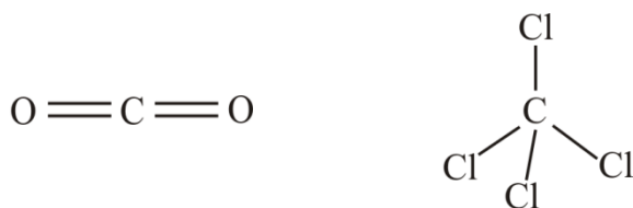
Figure 2.37 CO 2 and CCl 4 molecules
