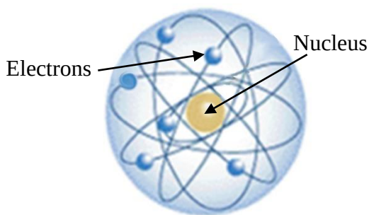
Figure 1.14 The Bohr model
