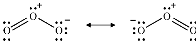
Figure 2.33 Resonance structures of O_3
