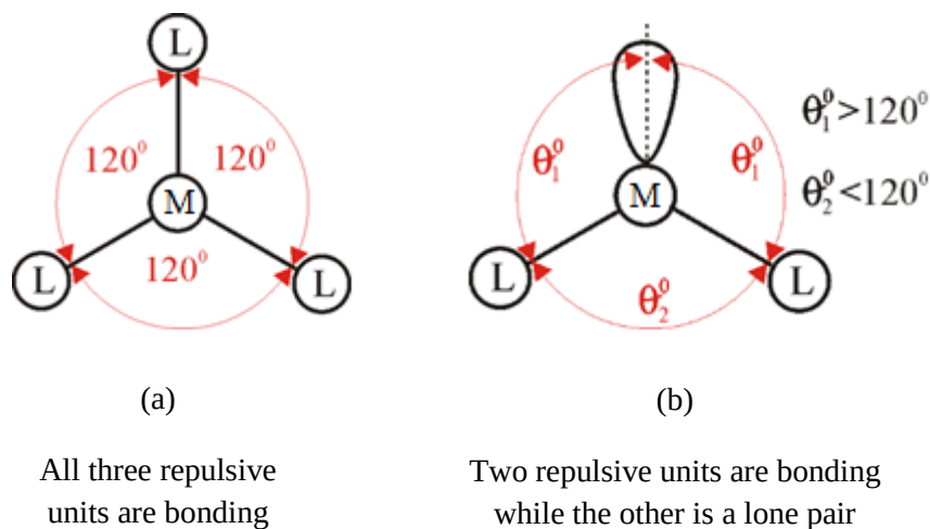
Figure 2.9 Trigonal planar electron pair geometry
