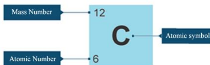
Figure 1.15 Atomic symbol of carbon
