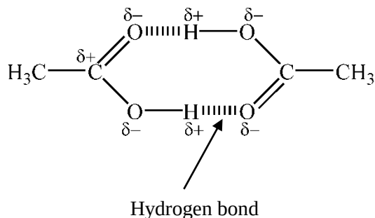
Figure 2.45 Hydrogen bonds in acetic acid
