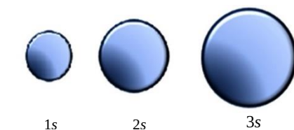
Figure 1.25 Shapes of the s orbitals
